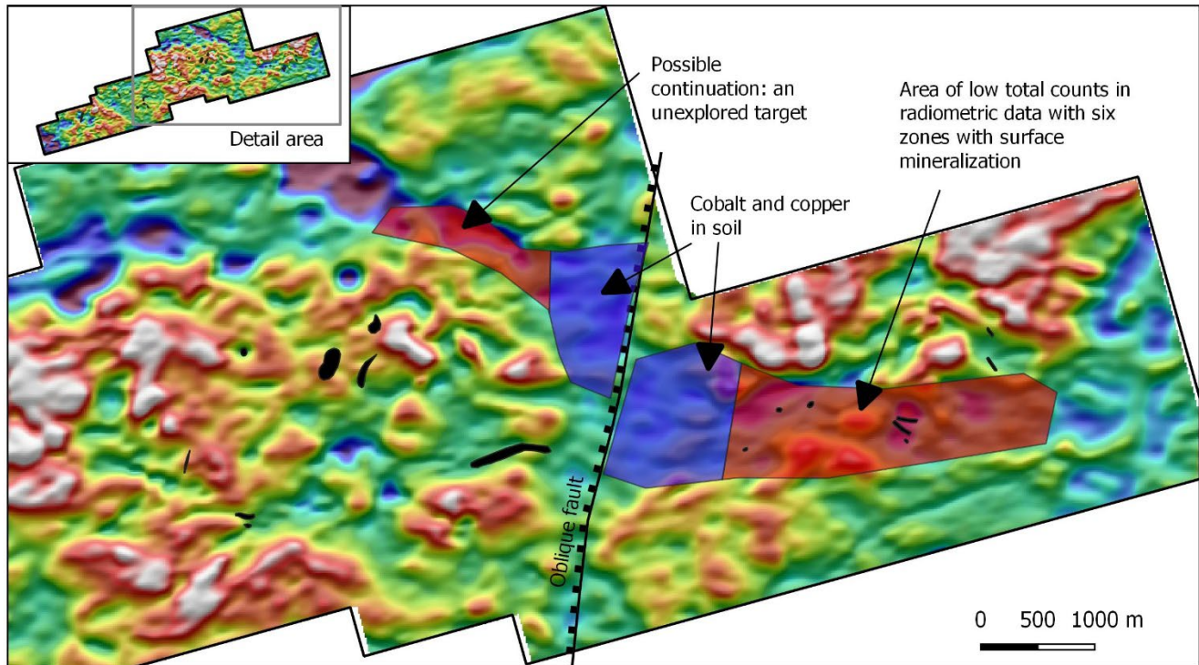
Figure 2. Total counts of radiometrics reveal a zone of low total counts that contains several surface showings in the east part of the property. The zone may continue to the north west as indicated by radiometric, soil, and spectral data.
