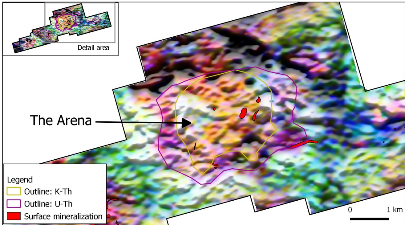
Figure 1. The Arena alteration zones overlain on a ternary map of K (red), Th (green) and U (blue), and shaded according to total counts.
